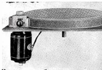
Presto 10-A turntable chassis only for mounting in existing cabinets.
