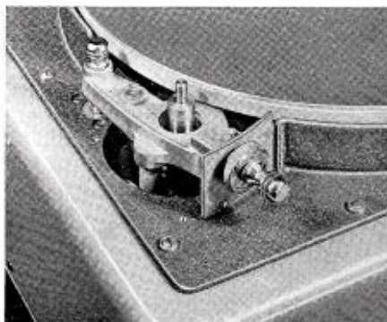
Unique Presto drive system. Step pulley on motor shaft drives against rubber tire on turntable rim. Lever changes speed instantly from 78 to 33½ RPM.
